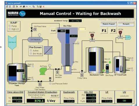
The Nulink Remote Monitoring and Management System enables full system control via PC or Smart Phone App.
